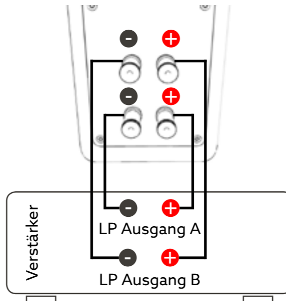
Bi-Wiring
